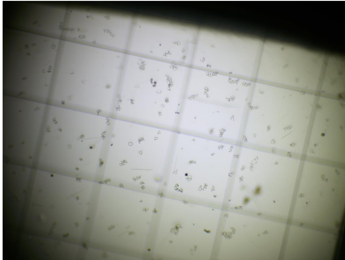
Photo 1. Shoreline at West Reservoir on July 28, 2026. Photo 2. Dolichospermum observed in water sample collected at West Reservoir on July 28, 2026.
